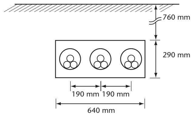
Detail 3 — 3 cables per phase
